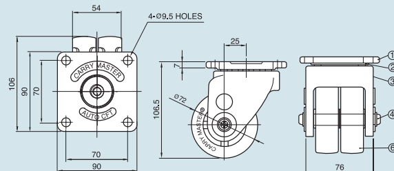
ACMT-800 Type
