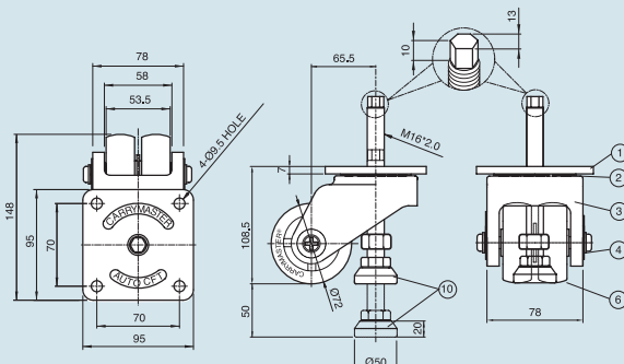
ALCT-1000F Type
