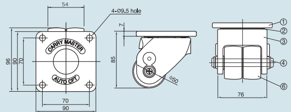
ACMT-600 Type
