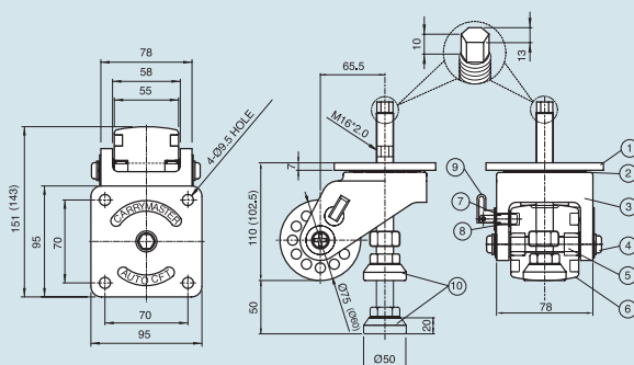
ALC-1000F Type
