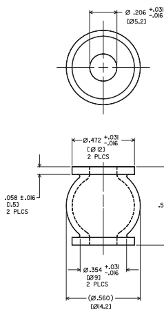
7110 Series Dimensional Drawing
